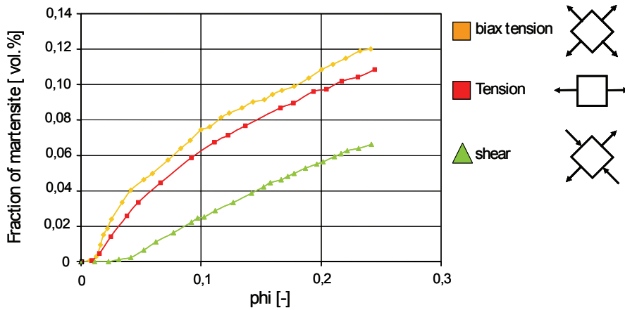
Fig. 4. Hardening of TRIP steels: Transformation of structure depends on stress [8]
