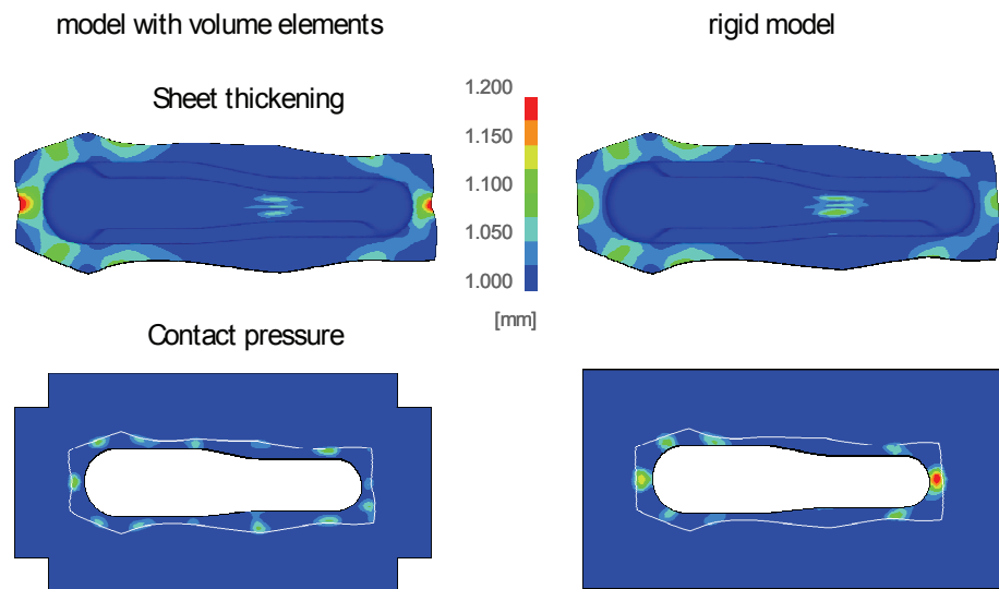
Fig. 11. Comparison simulation with rigid and elastic die models
