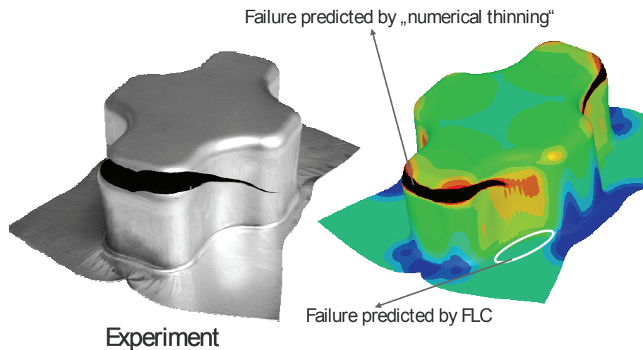
Fig. 9. Prediction of Failure – Cross Die (TRIP 700)
