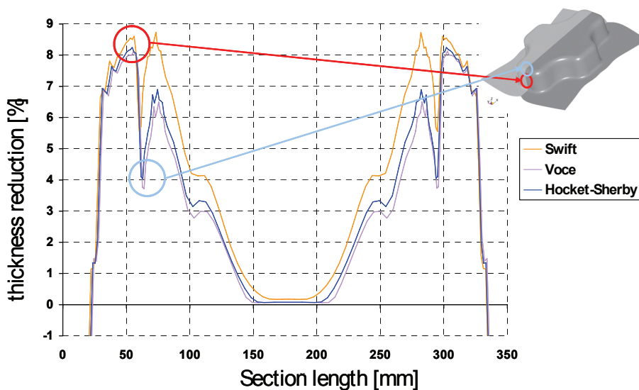
Fig. 6. Effect of flow-curve approximation on the simulation result
