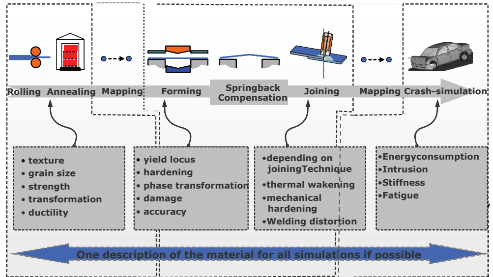
Fig. 12. Schematic overview of the future simulation environment
