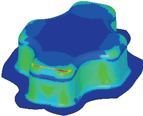
Fig. 10. Simulation of Cross-die formability test using GISSMO coupled to Barlat-Model; left: experiment, right: predicted failure
