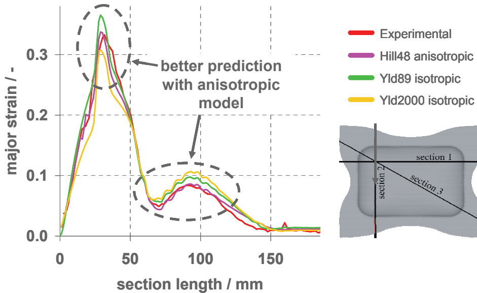
Fig. 8. Anisotropic hardening, distribution of major strain (along section 3)
