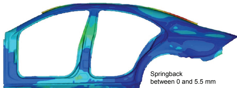
Fig. 2. Springback simulation of a sidewall
