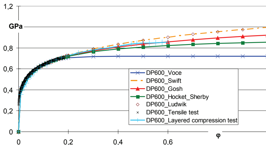
Fig. 5. Yield Curves - Method of Extrapolation, Material Steel DP600
