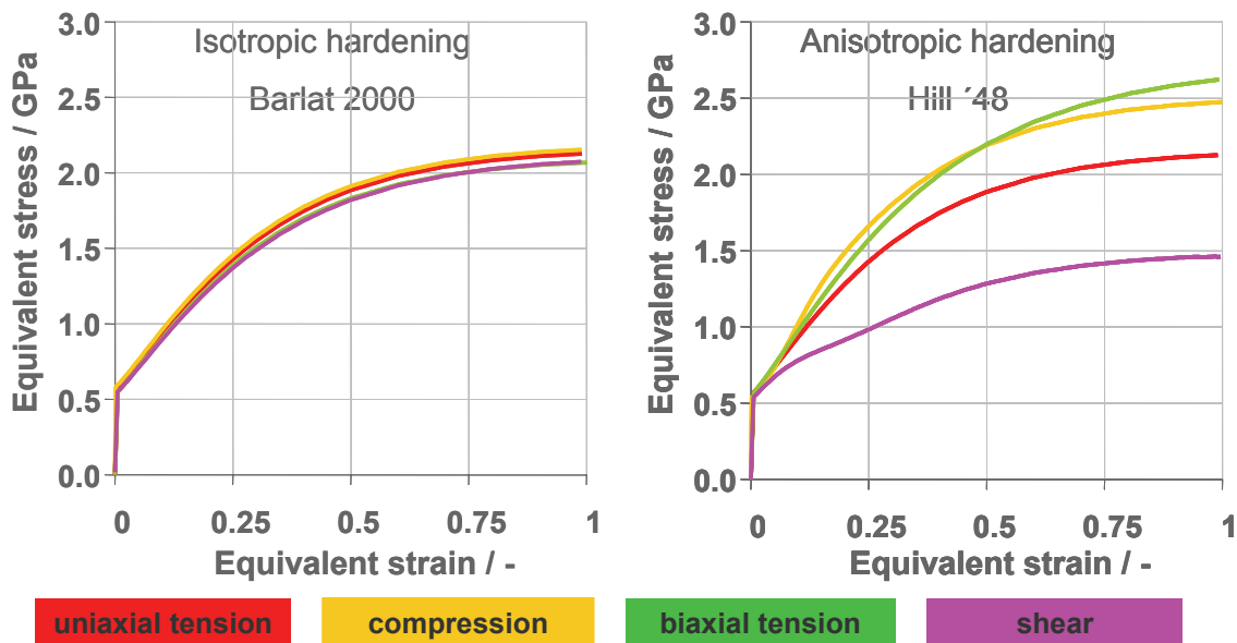
Fig. 7. Yield curve comparison for different load paths
